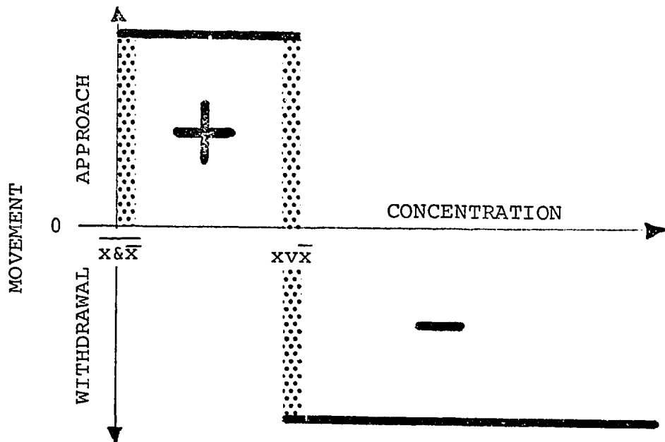
Fig. 2. The laws of "excluded contradiction" ( \overline{x \ \& \ \bar{x}} ) and of "excluded middle" ( x \vee \bar{x} ) in the twilight zones between no motion ( M = 0 ) and approach (+), and between approach (+) and withdrawal (-) as a function of the concentration (C) of a perceptible agent.
