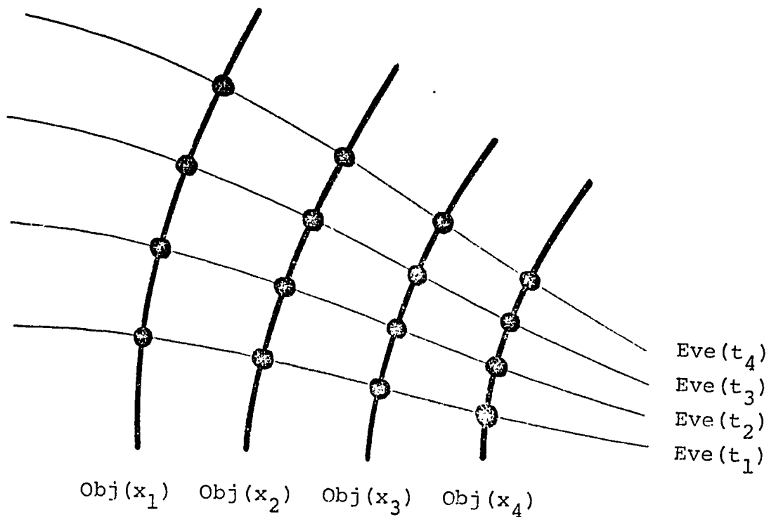
Fig. 1. "Objects" creating "Events" and vice versa .
